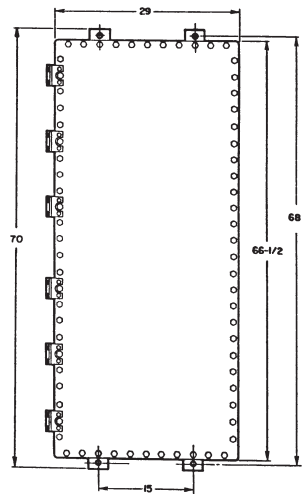
Enclosure
