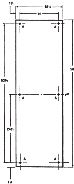
Mounting plate
