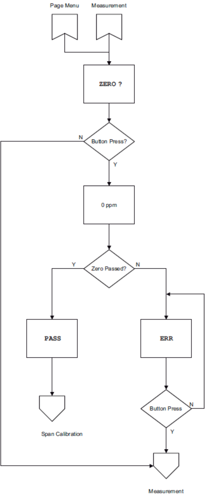
Figure 11 Zero calibration
