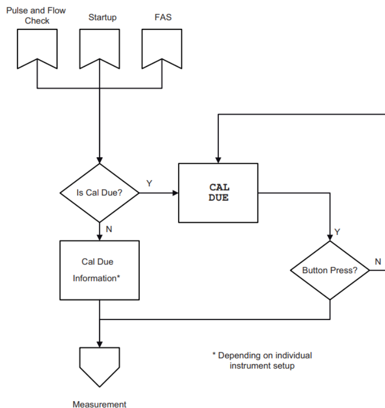
Figure 7 Calibration due
