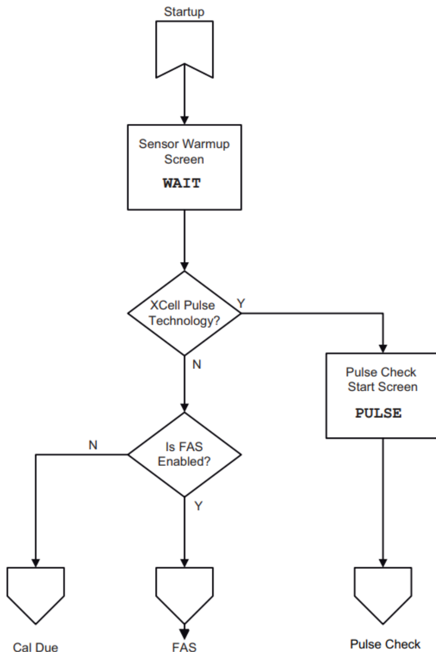
Figure 4 Startup, continued
