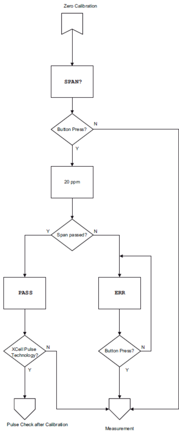
Figure 12 Span calibration
