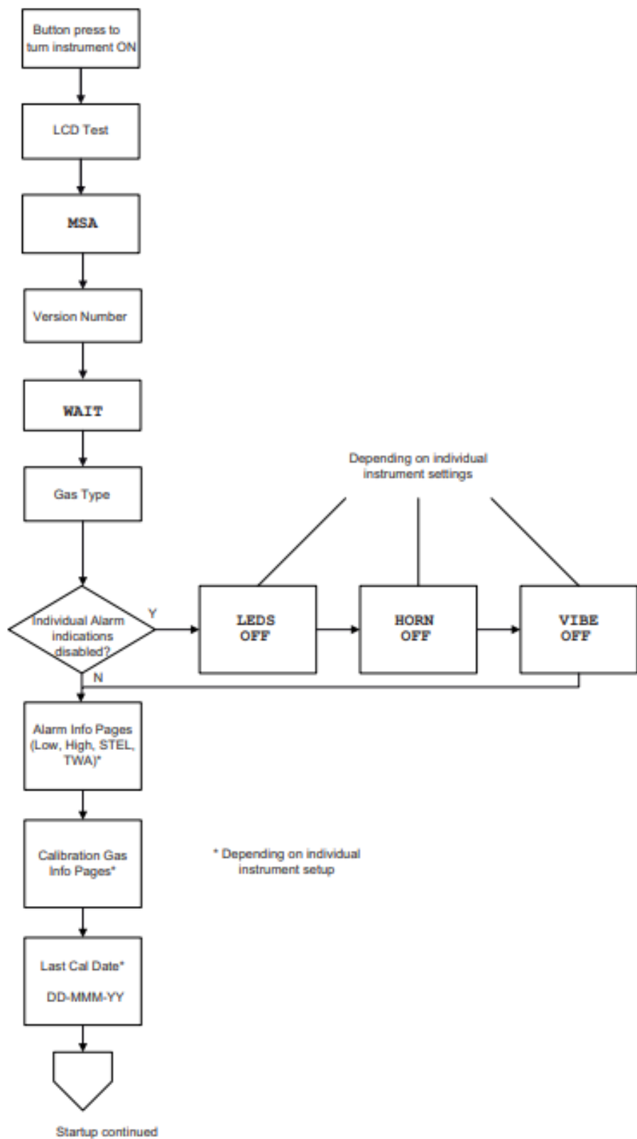
Figure 3 Startup
