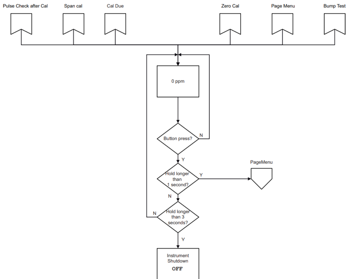
Figure 8 Measurement
