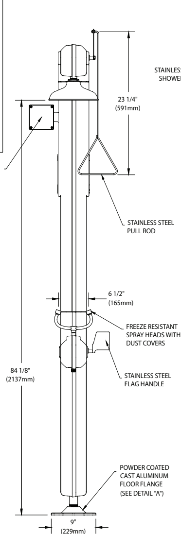
HEAT TRACE POWER CONNECTION BOX
