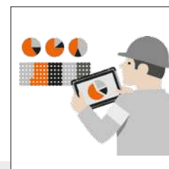
Workflow Management/SAP
